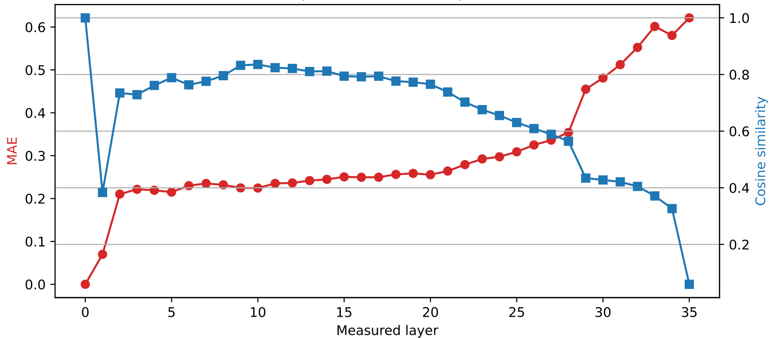
SmolLM3-3B | Quantized layer 0 | float16 \rightarrow int2
