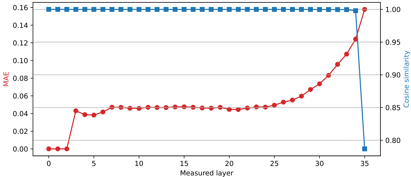
SmolLM3-3B | Quantized layer 2 | float16 \rightarrow int2
