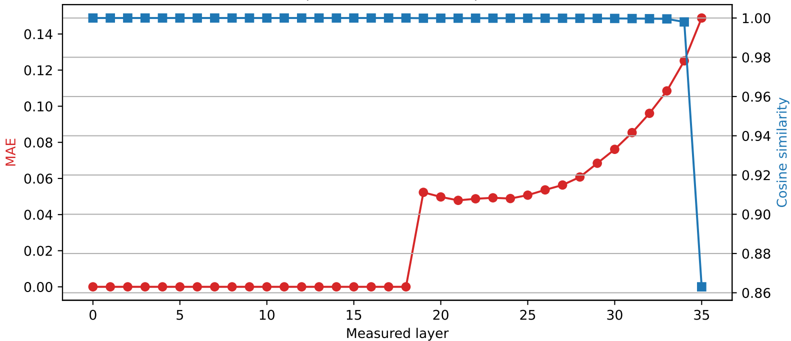
SmolLM3-3B | Quantized layer 18 | float16 \rightarrow int2
