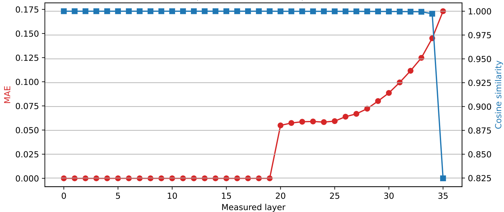
SmolLM3-3B | Quantized layer 19 | float16 → int2
