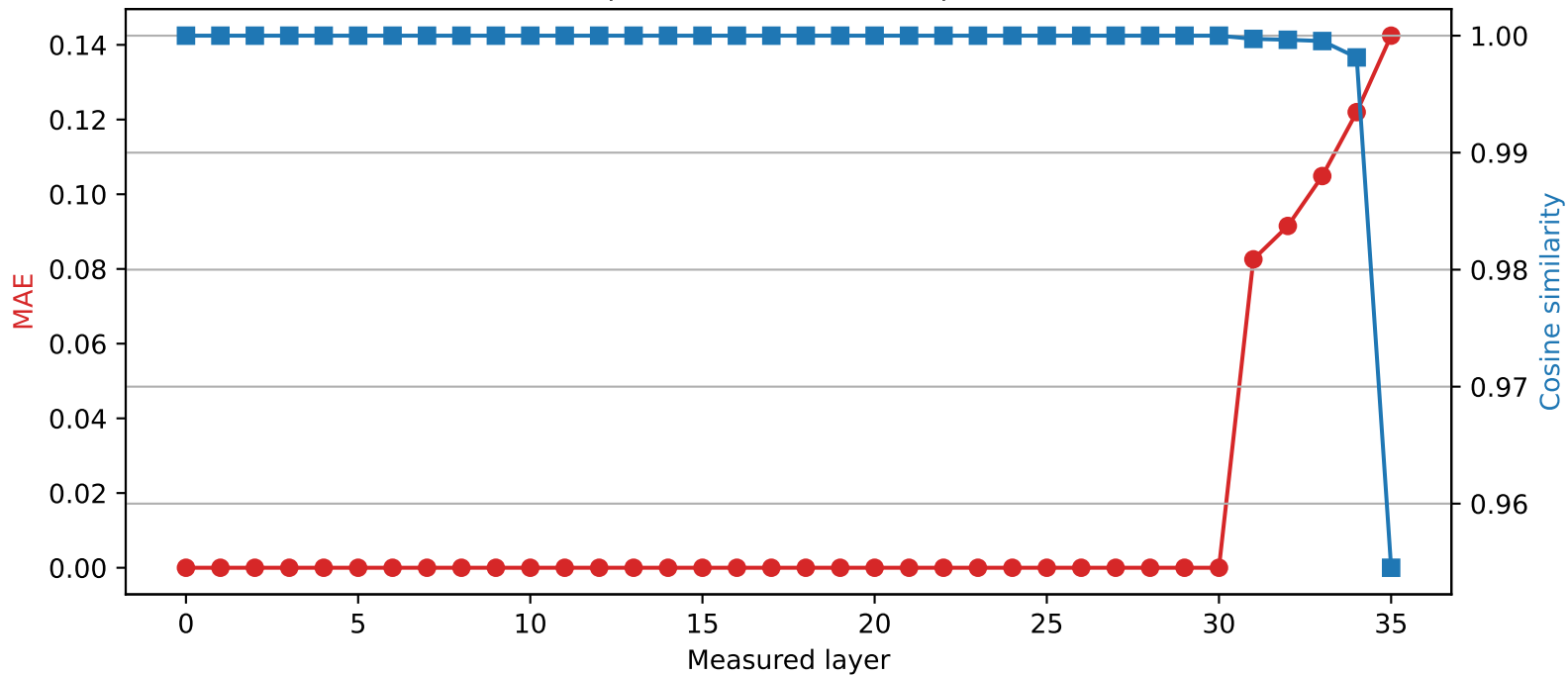
SmolLM3-3B | Quantized layer 30 | float16 \rightarrow int2
