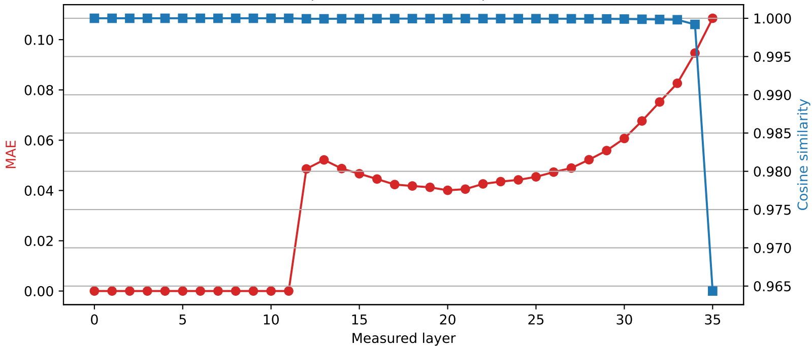
SmolLM3-3B | Quantized layer 11 | float16 → int2
