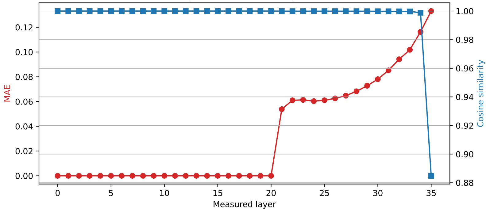
SmolLM3-3B | Quantized layer 20 | float16 → int2
