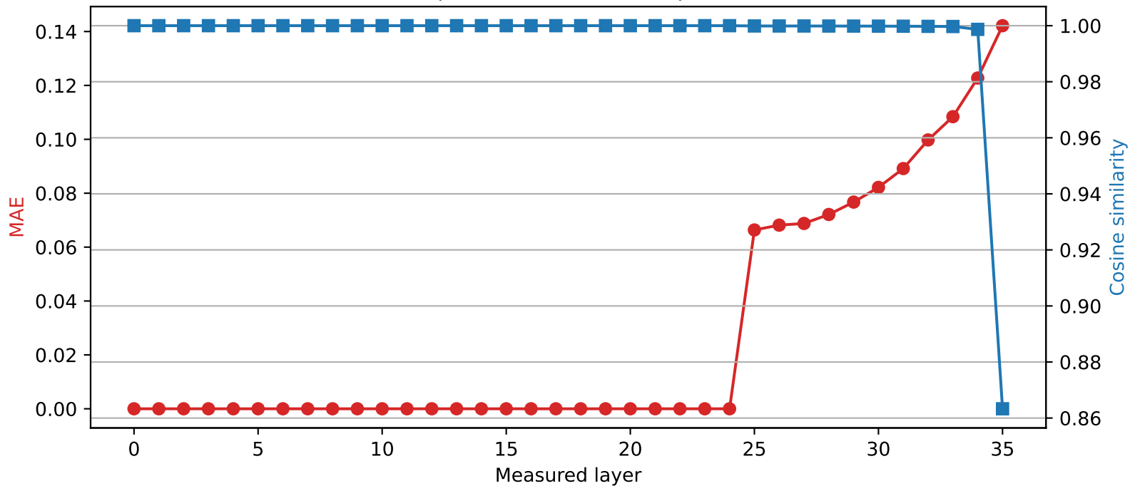
SmolLM3-3B | Quantized layer 24 | float16 \rightarrow int2
