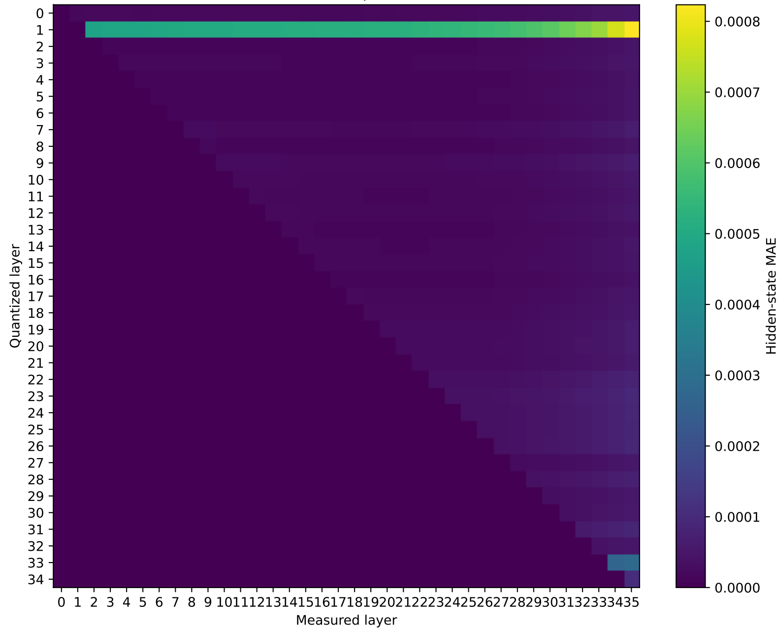
Model: SmolLM3-3B | float32 → int16
