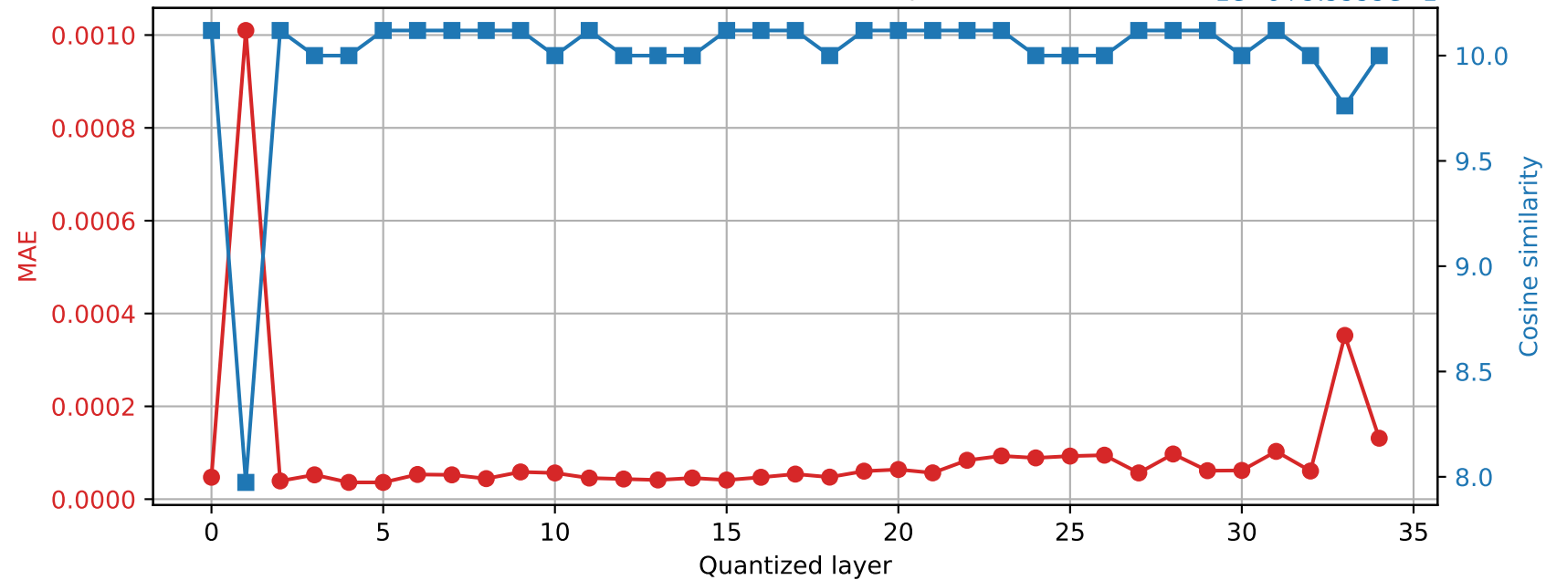
SmolLM3-3B | Prompt 0 Final RMSNorm output damage | float32 \rightarrow int16
