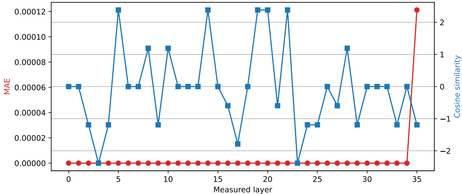
SmolLM3-3B | Quantized layer 34 | float32 \rightarrow int16
