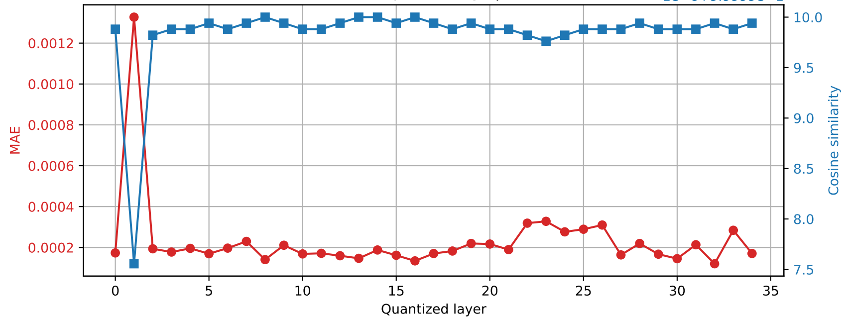
SmolLM3-3B | Prompt 1 Final RMSNorm output damage | float32 → int16
