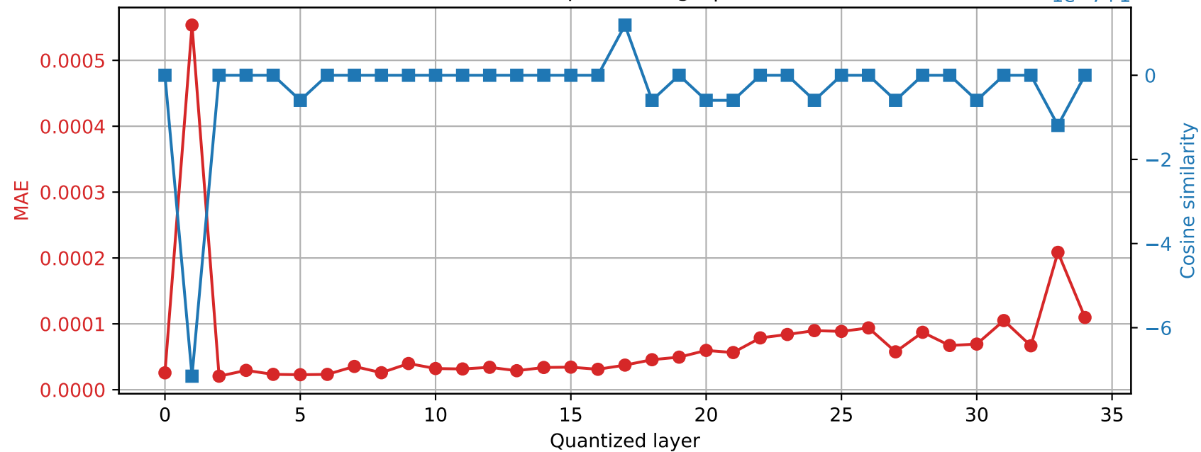
SmolLM3-3B | Prompt 2 Final RMSNorm output damage | float32 → int16
