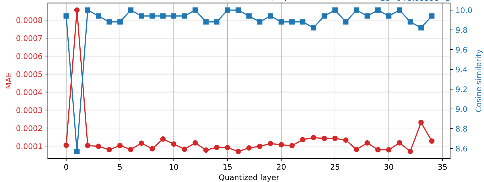
SmolLM3-3B | Prompt 3 Final RMSNorm output damage | float32 → int16
