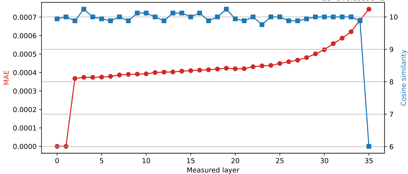
SmolLM3-3B | Quantized layer 1 | float32 \rightarrow int16 1e-6+9.9999e-1
