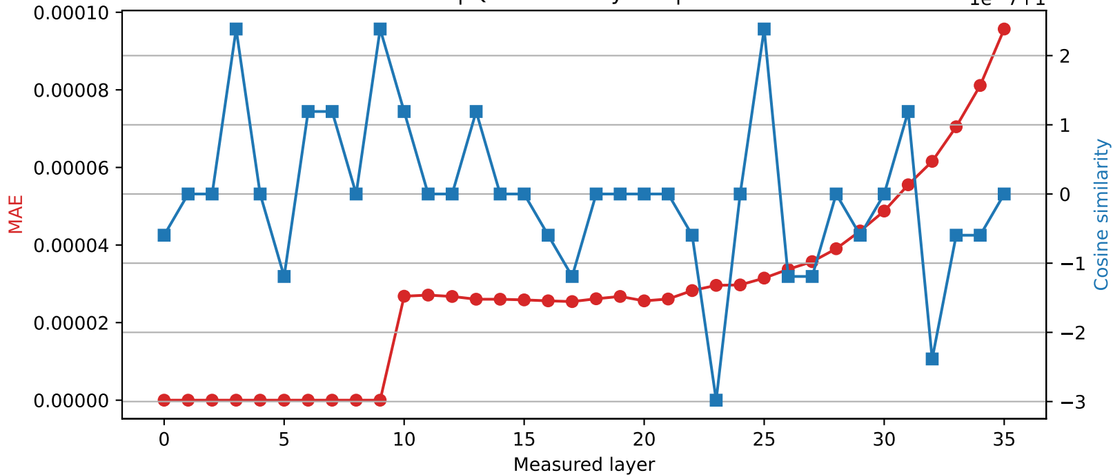
SmolLM3-3B | Quantized layer 9 | float32 → int16
