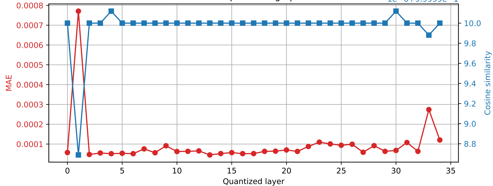
SmolLM3-3B | Prompt 4 Final RMSNorm output damage | float32 → int16
