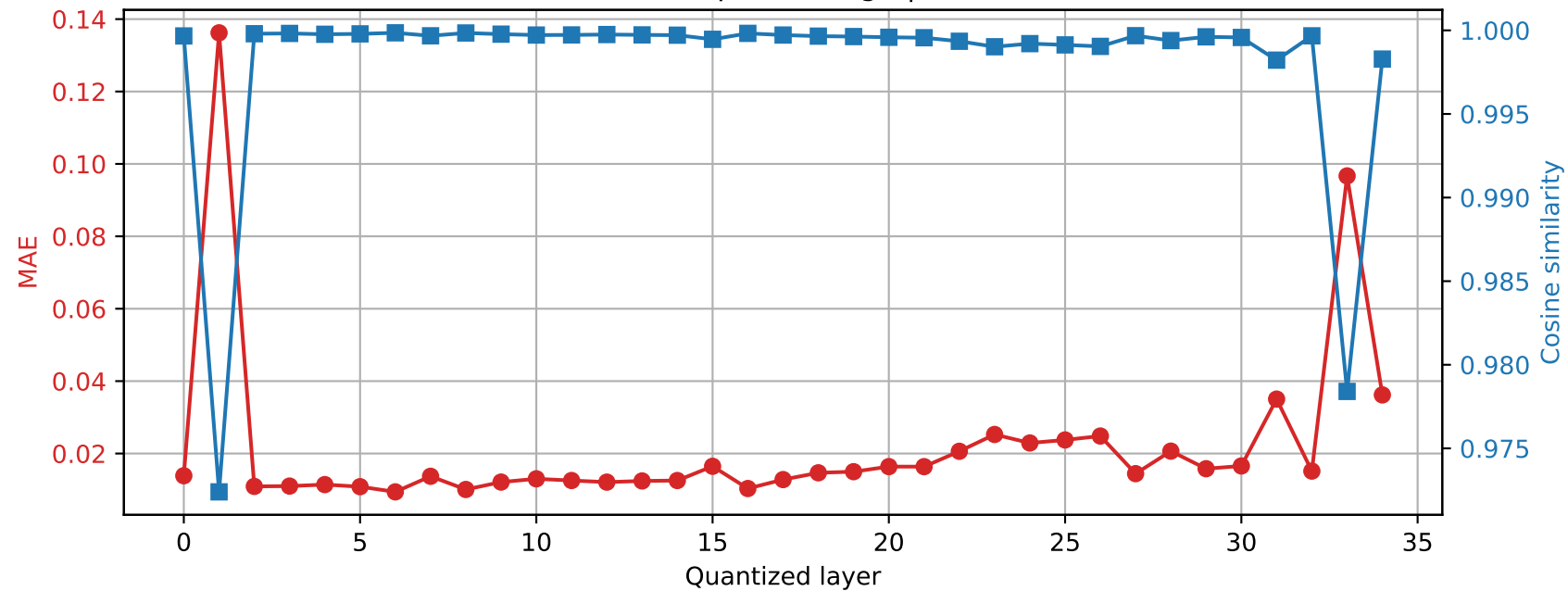
SmolLM3-3B | Prompt 0 Final RMSNorm output damage | float32 \rightarrow int8
