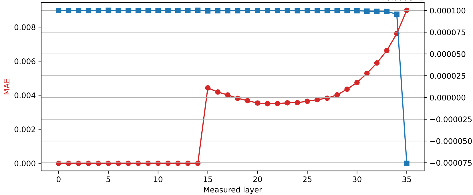
SmolLM3-3B | Quantized layer 14 | float32 → int8
