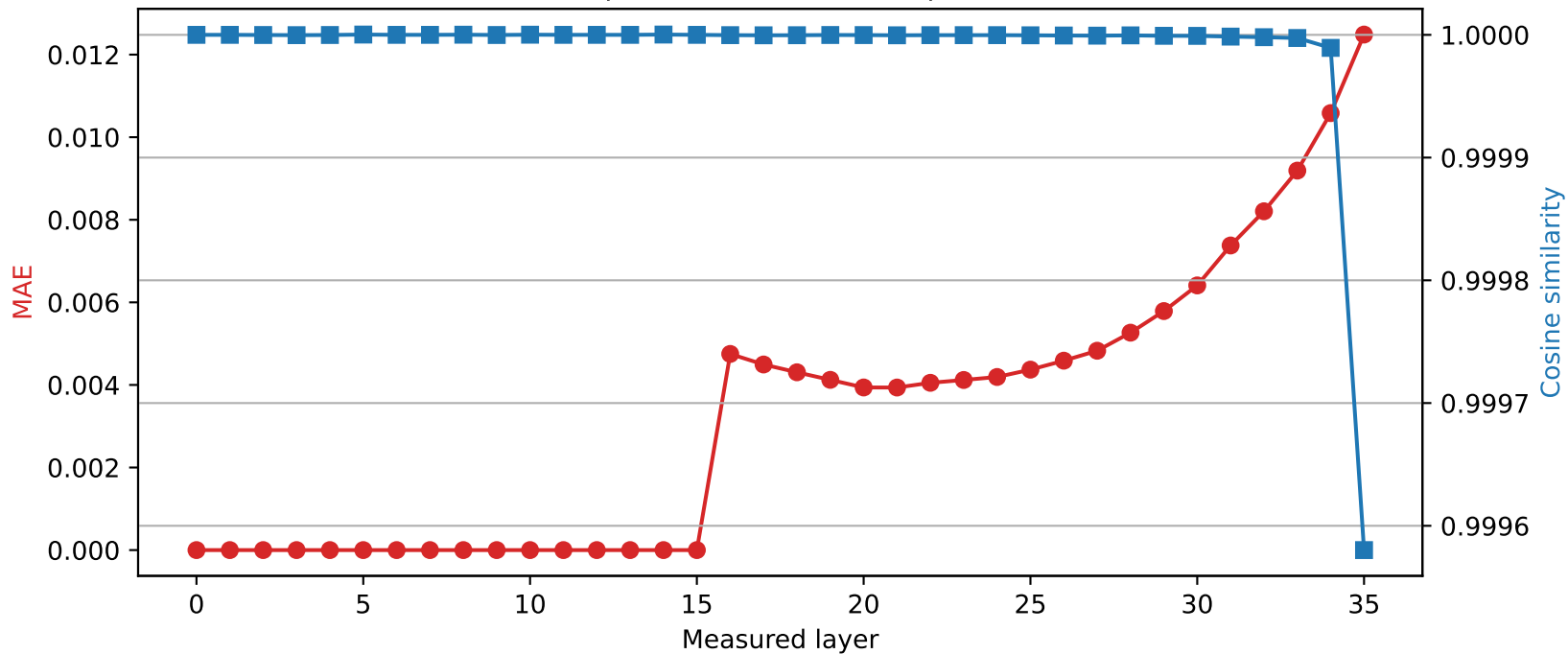
SmolLM3-3B | Quantized layer 15 | float32 → int8
