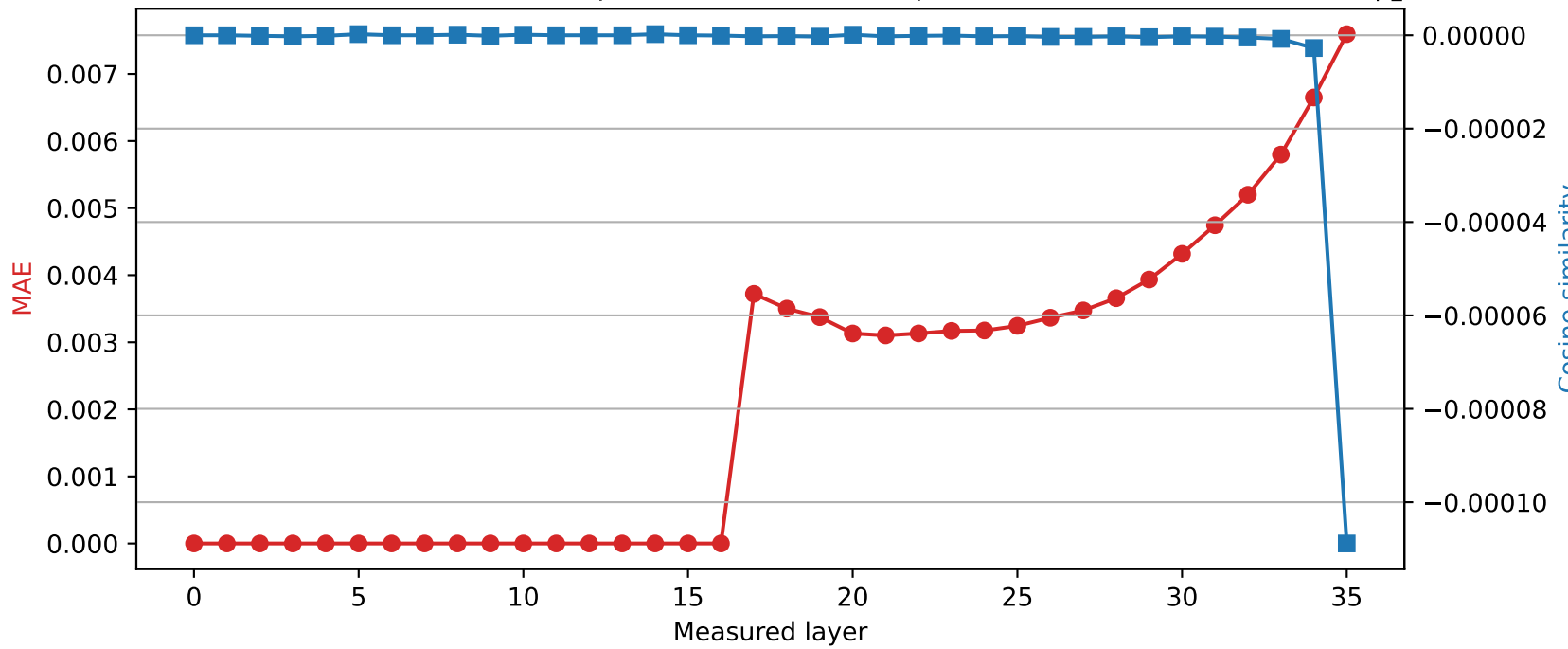
SmolLM3-3B | Quantized layer 16 | float32 \rightarrow int8
