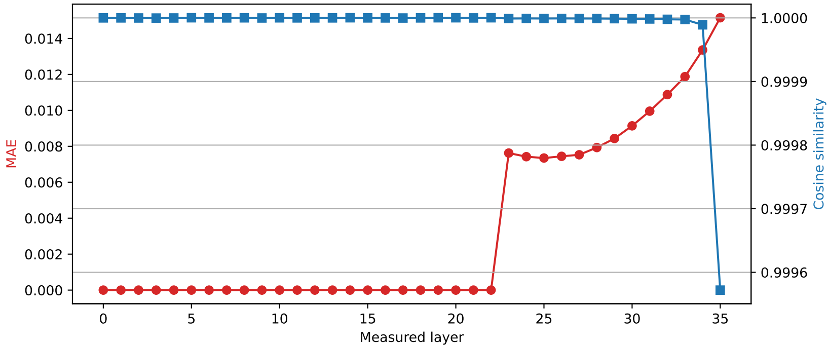
SmolLM3-3B | Quantized layer 22 | float32 \rightarrow int8
