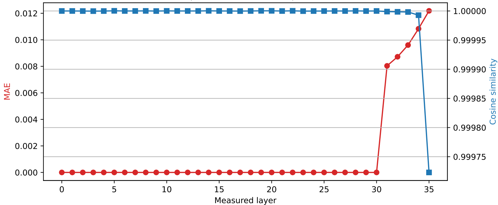
SmolLM3-3B | Quantized layer 30 | float32 \rightarrow int8
