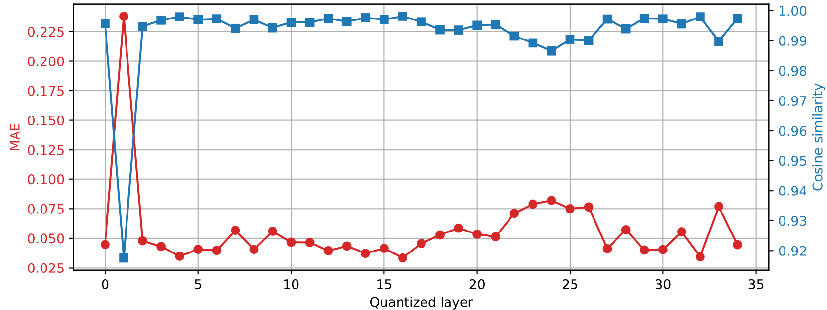
SmolLM3-3B | Prompt 1 Final RMSNorm output damage | float32 \rightarrow int8
