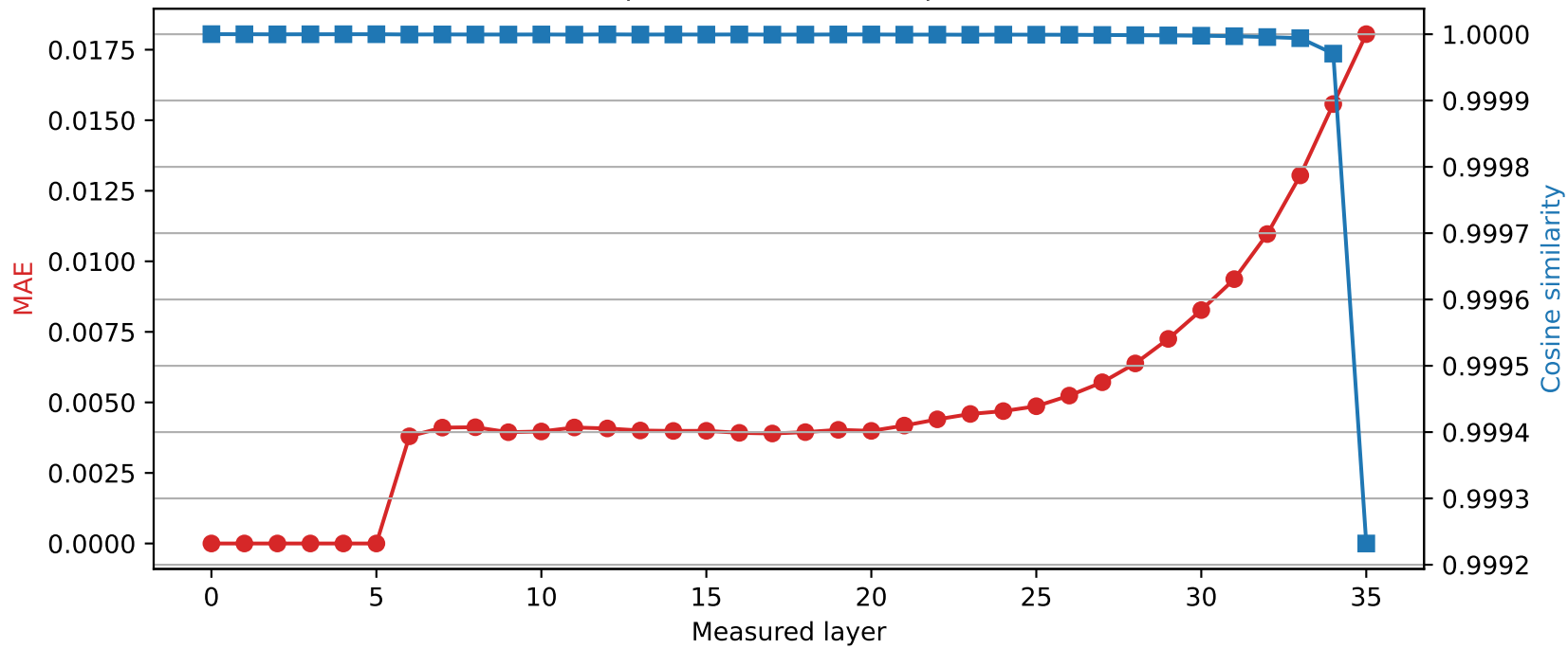
SmolLM3-3B | Quantized layer 5 | float32 \rightarrow int8
