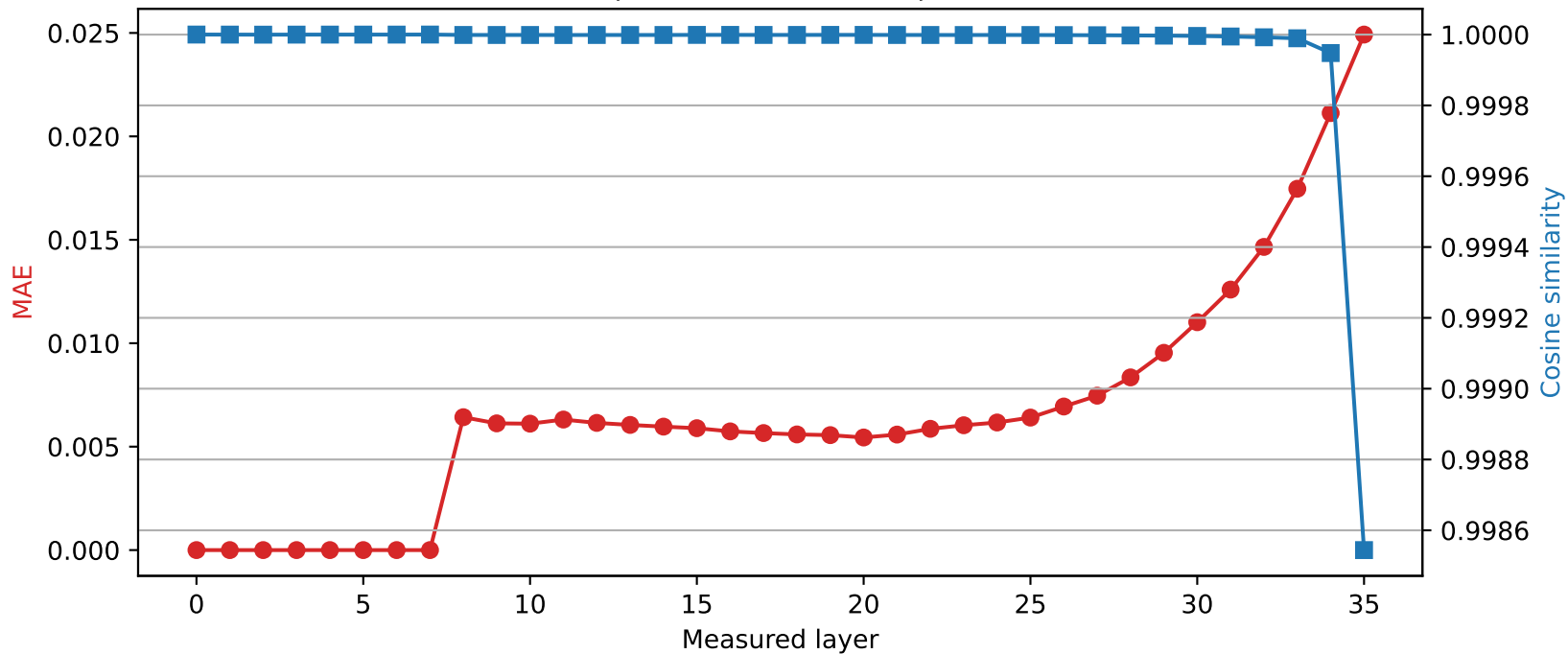
SmolLM3-3B | Quantized layer 7 | float32 \rightarrow int8
