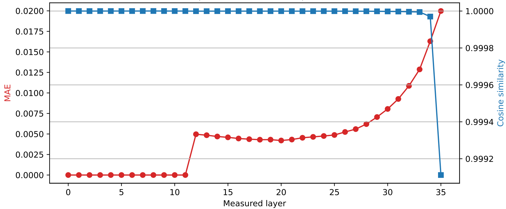
SmolLM3-3B | Quantized layer 11 | float32 \rightarrow int8
