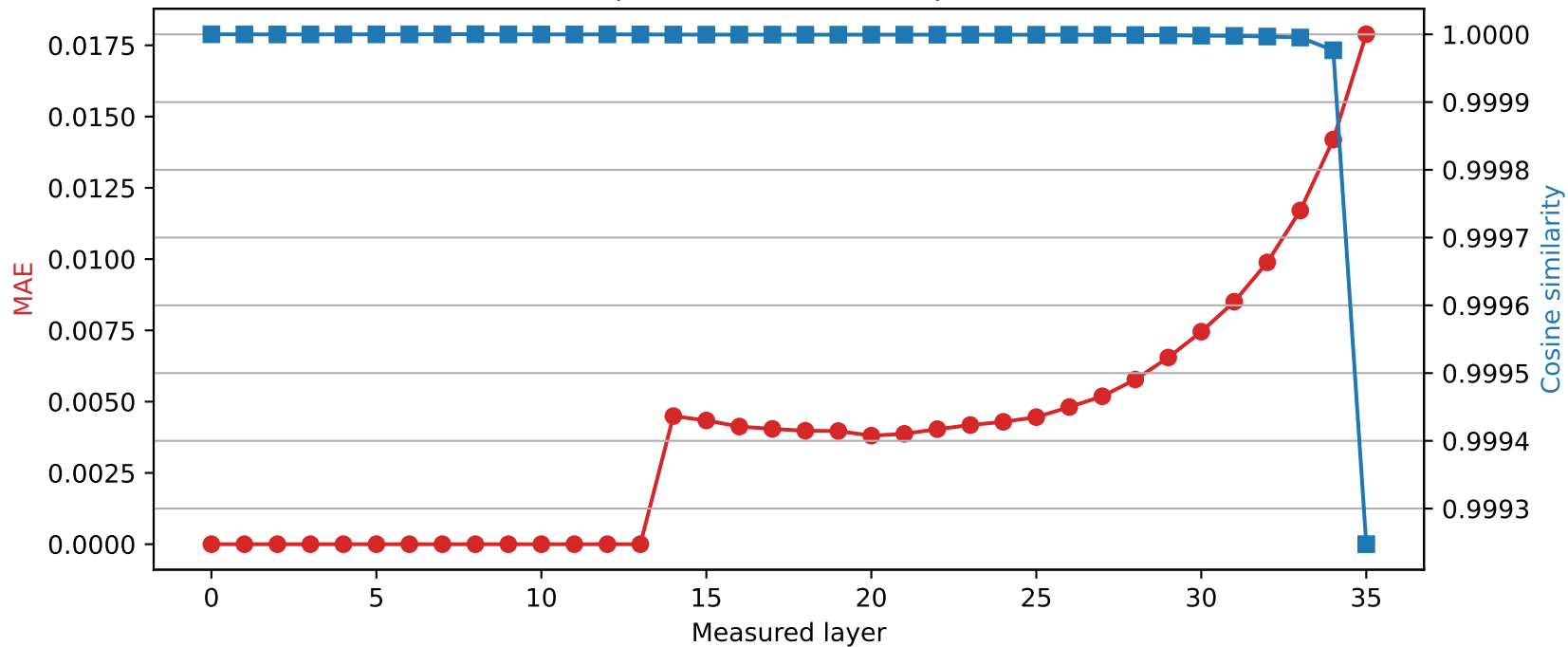
SmolLM3-3B | Quantized layer 13 | float32 \rightarrow int8
