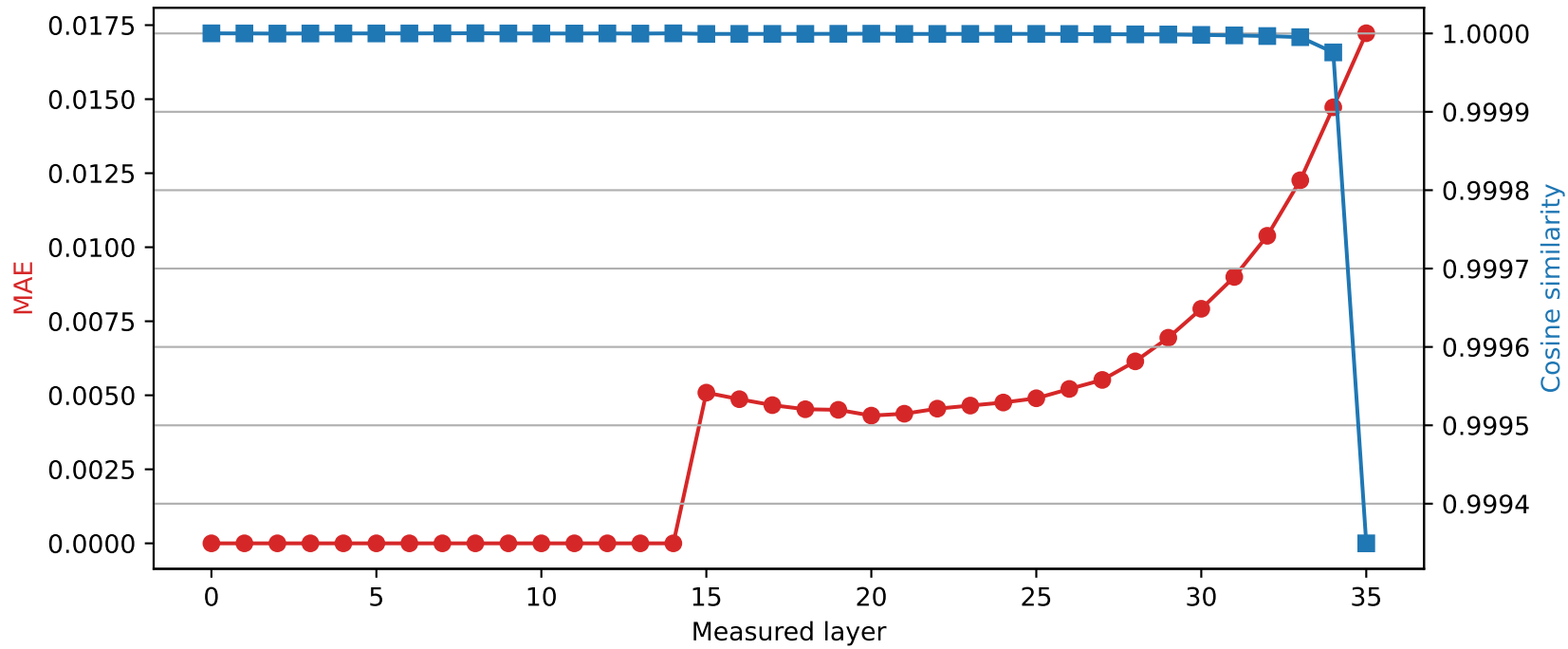
SmolLM3-3B | Quantized layer 14 | float32 \rightarrow int8
