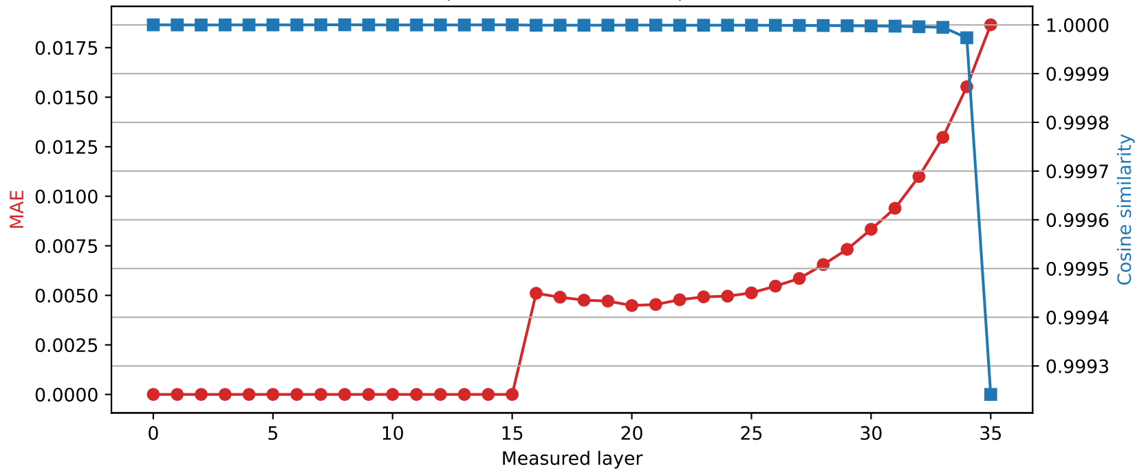
SmolLM3-3B | Quantized layer 15 | float32 \rightarrow int8
