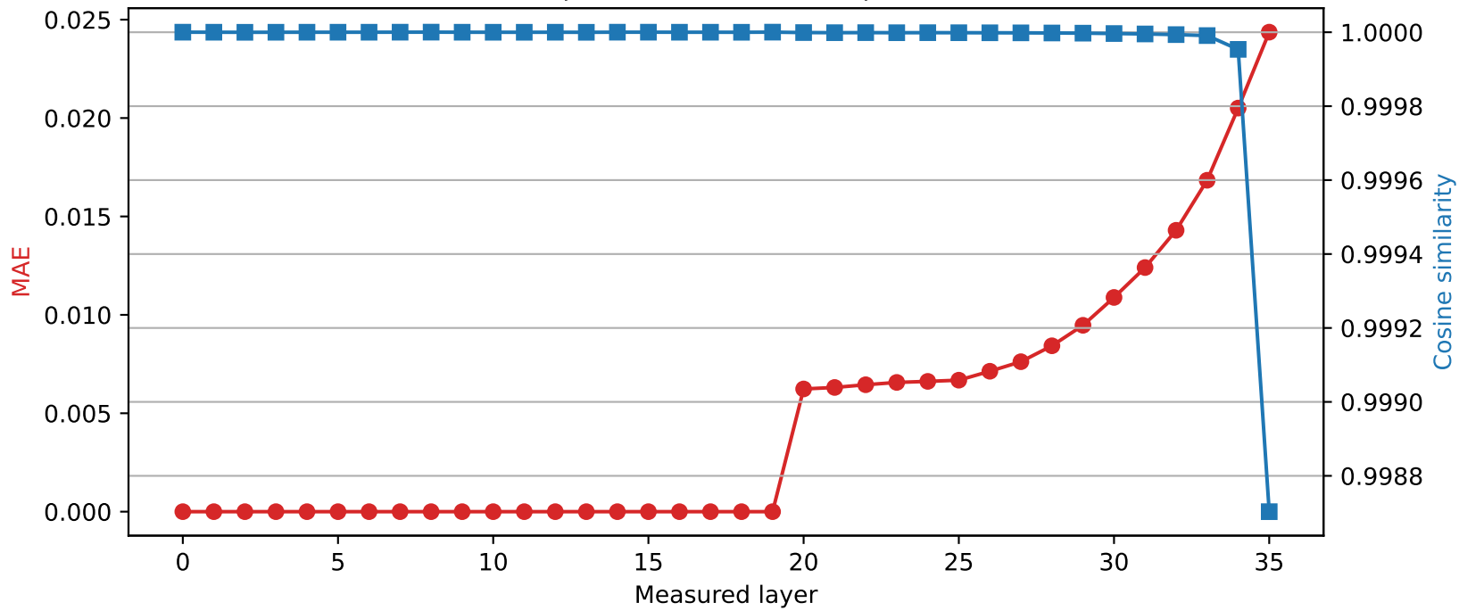
SmolLM3-3B | Quantized layer 19 | float32 \rightarrow int8
