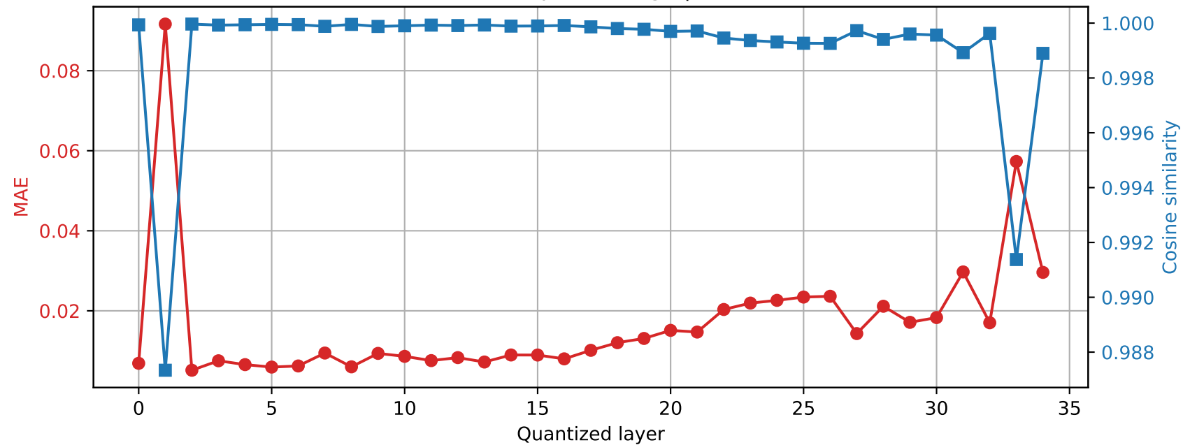
SmolLM3-3B | Prompt 2 Final RMSNorm output damage | float32 → int8
