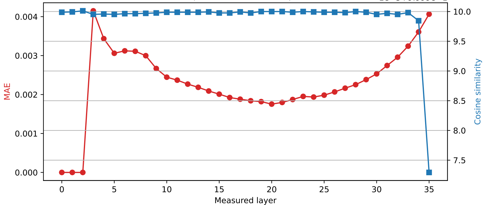
SmolLM3-3B | Quantized layer 2 | float32 → int8
