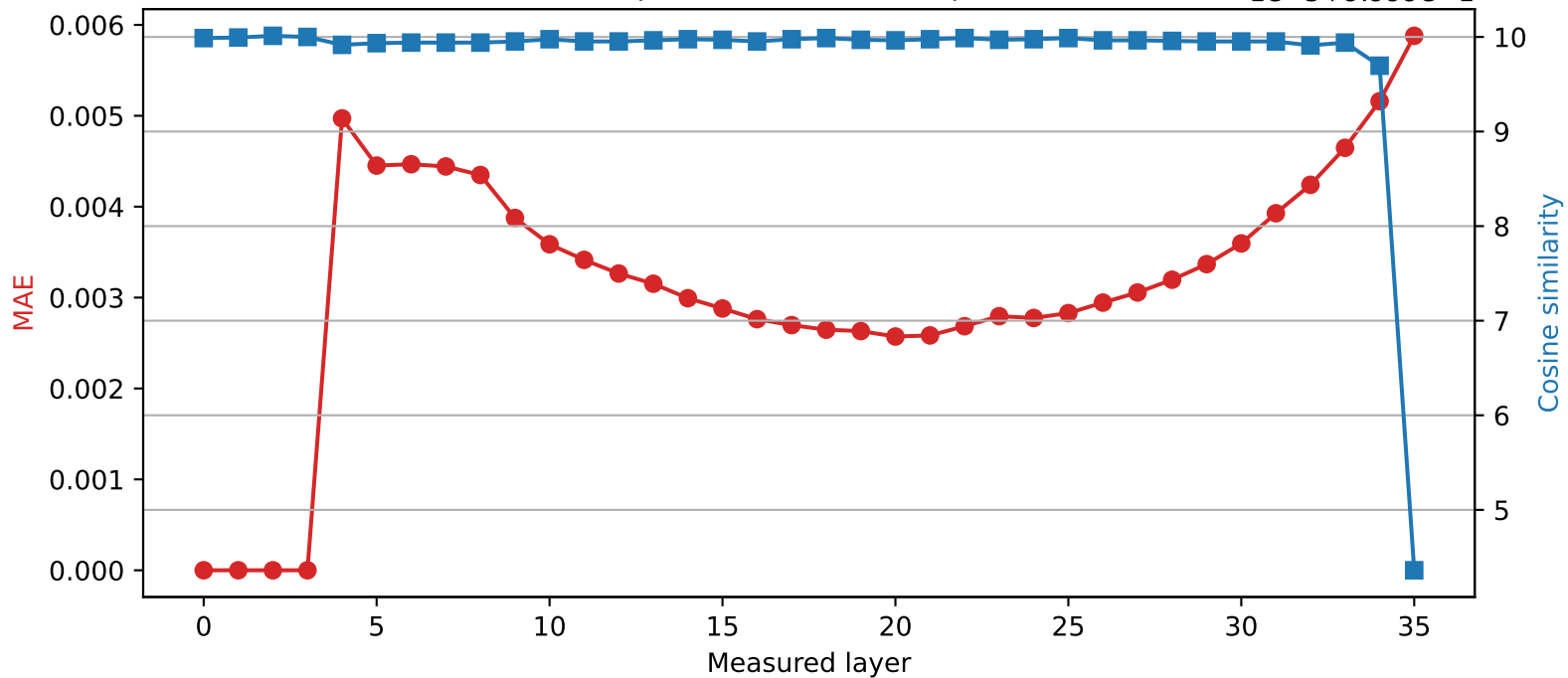
SmolLM3-3B | Quantized layer 3 | float32 → int8
