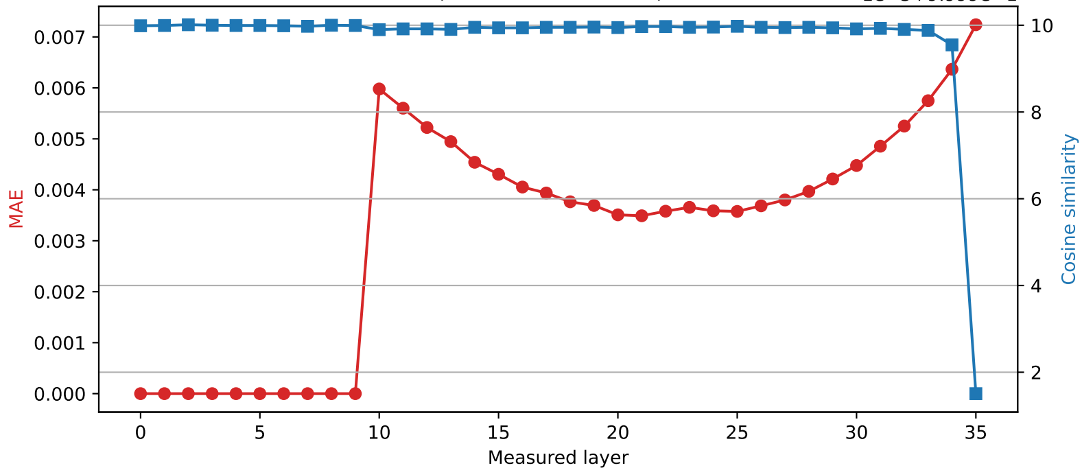
SmolLM3-3B | Quantized layer 9 | float32 \rightarrow int8
