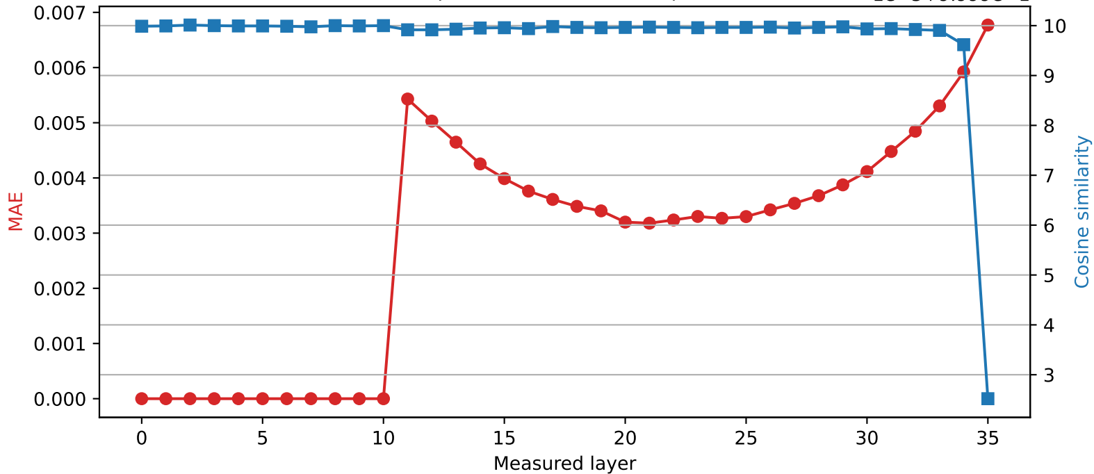
SmolLM3-3B | Quantized layer 10 | float32 → int8
