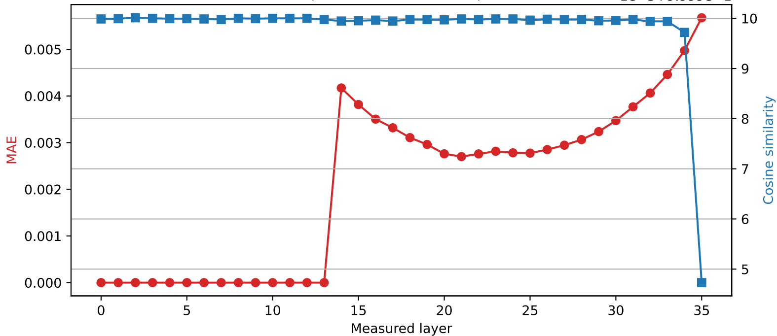
SmolLM3-3B | Quantized layer 13 | float32 → int8
