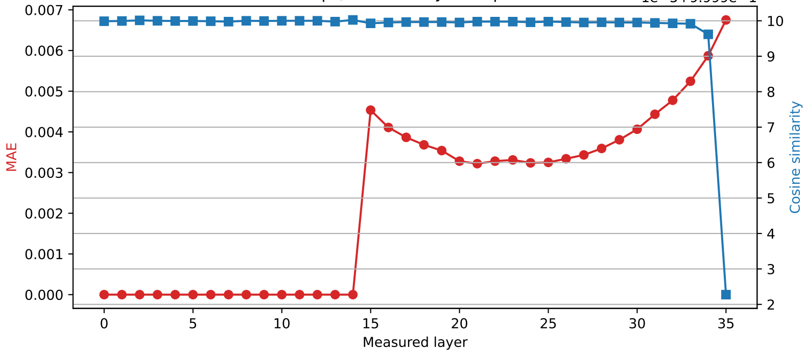
SmolLM3-3B | Quantized layer 14 | float32 → int8
