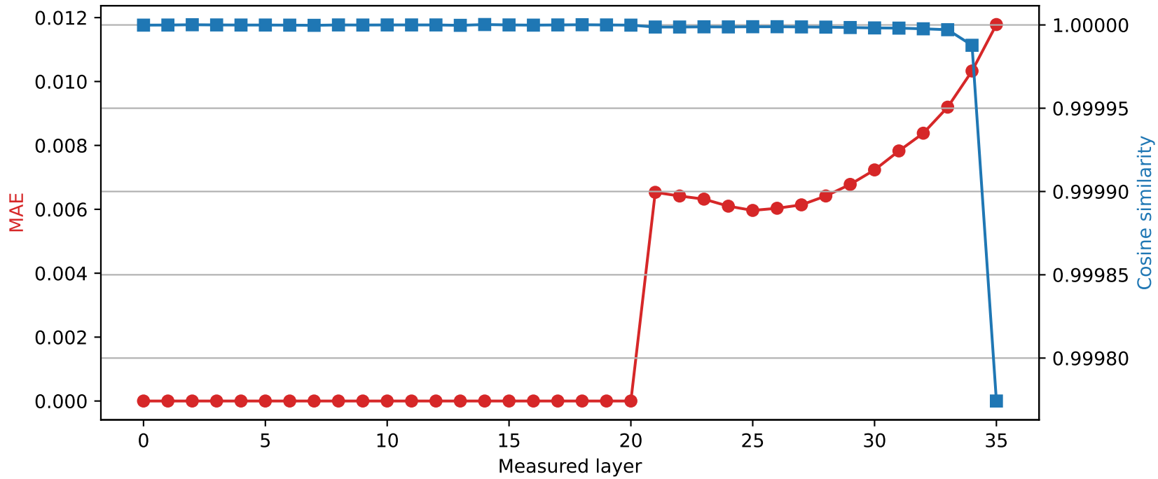
SmolLM3-3B | Quantized layer 20 | float32 \rightarrow int8
