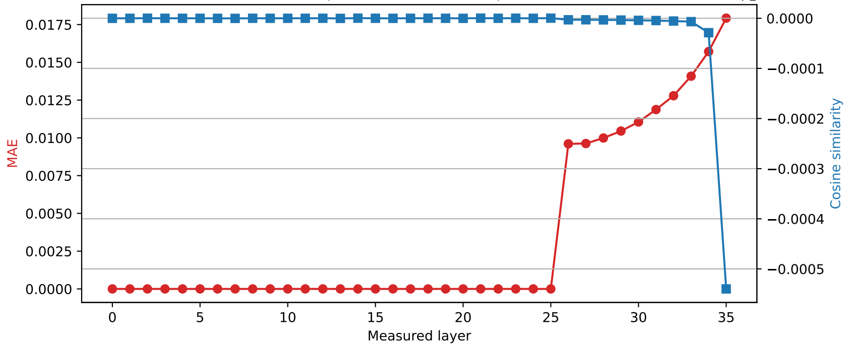
SmolLM3-3B | Quantized layer 25 | float32 \rightarrow int8
