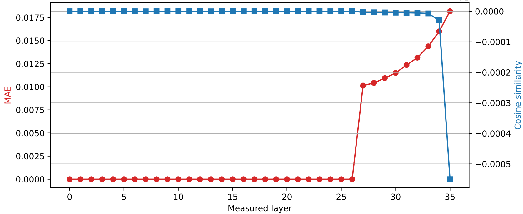
SmolLM3-3B | Quantized layer 26 | float32 \rightarrow int8
