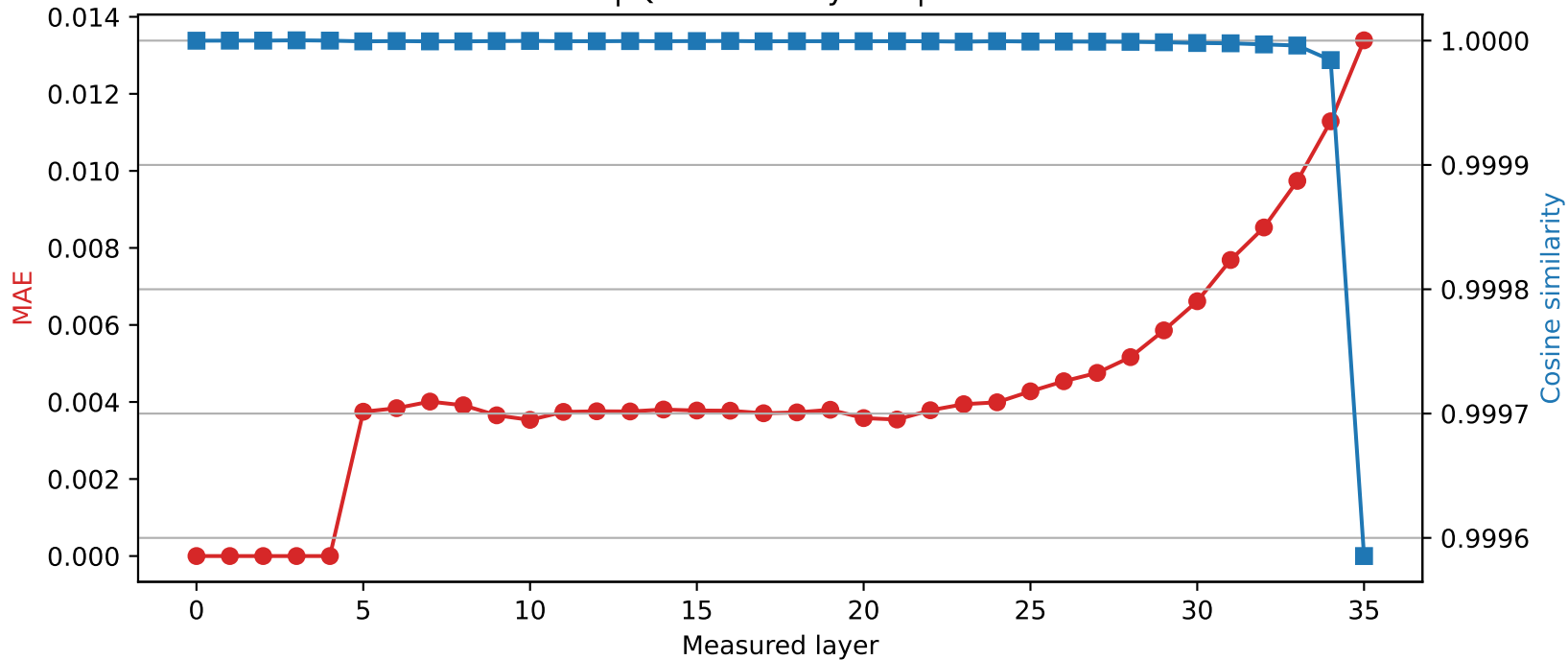
SmolLM3-3B | Quantized layer 4 | float32 \rightarrow int8
