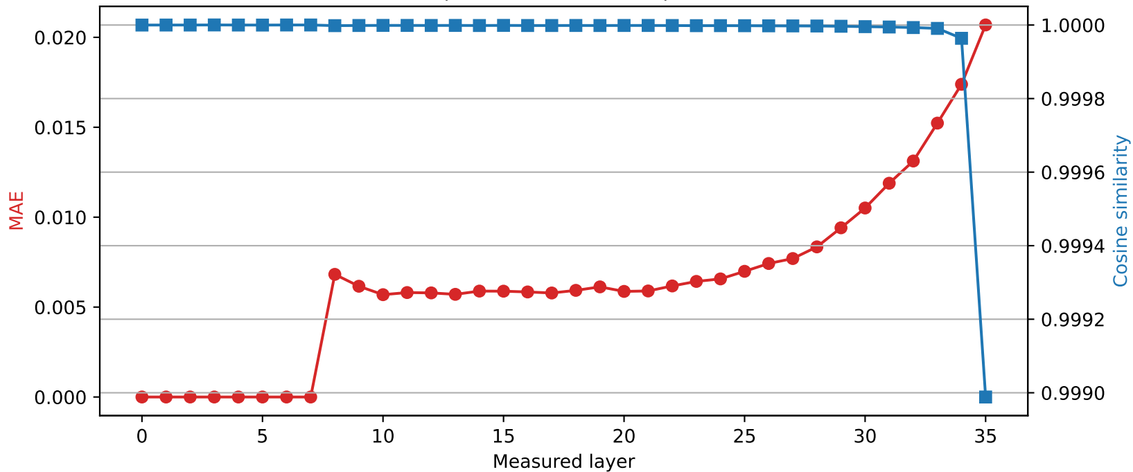
SmolLM3-3B | Quantized layer 7 | float32 → int8
