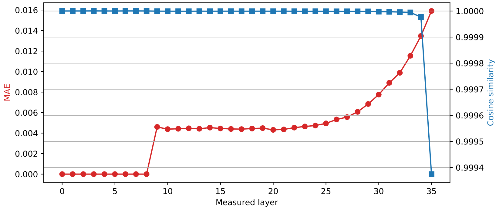
SmolLM3-3B | Quantized layer 8 | float32 \rightarrow int8
