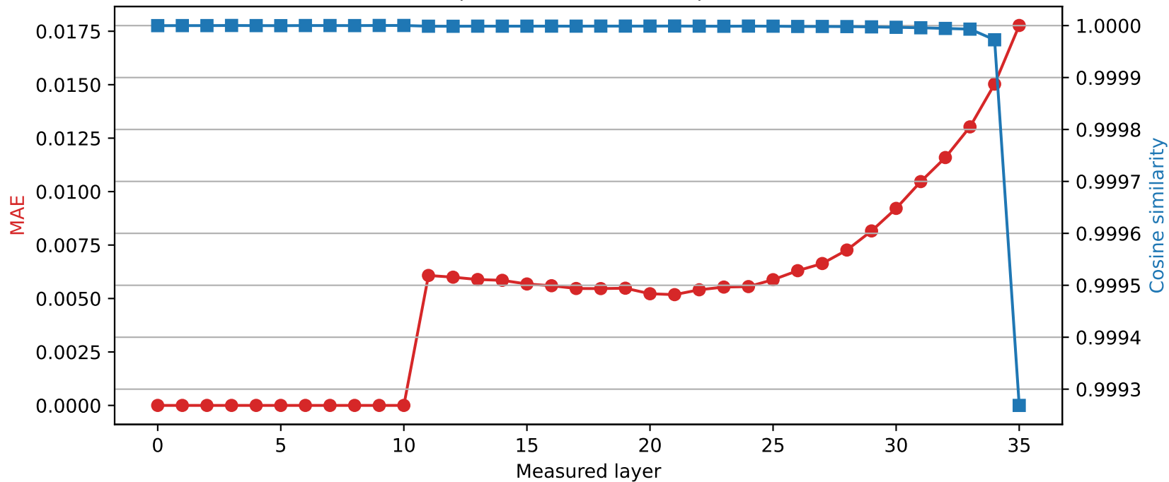
SmolLM3-3B | Quantized layer 10 | float32 \rightarrow int8
