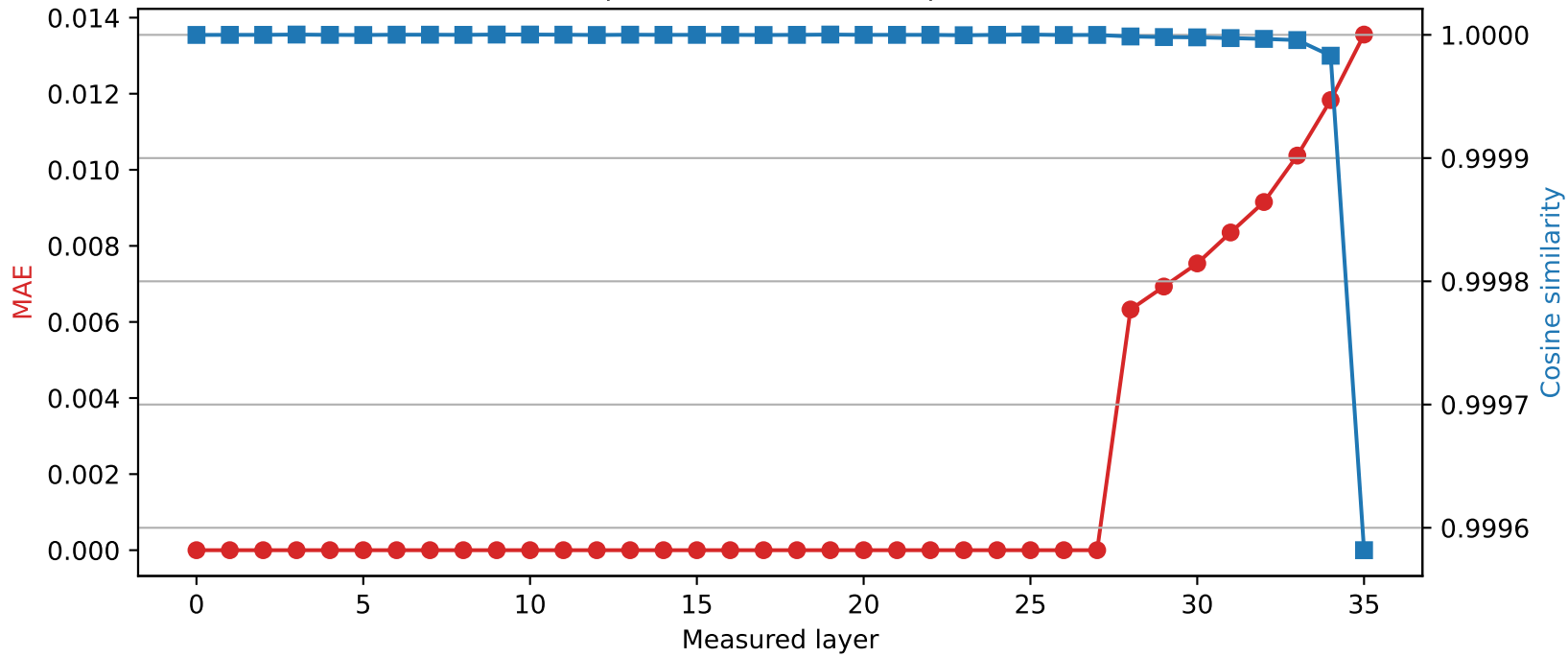
SmolLM3-3B | Quantized layer 27 | float32 \rightarrow int8
