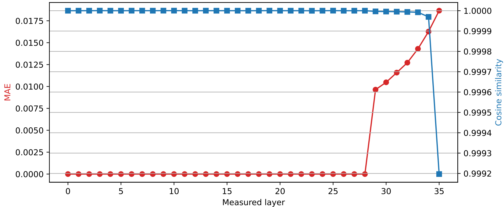
SmolLM3-3B | Quantized layer 28 | float32 → int8
