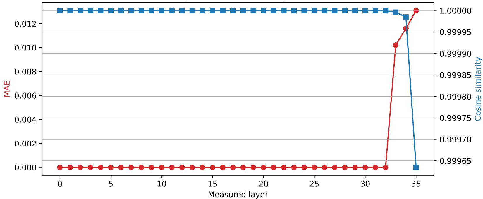
SmolLM3-3B | Quantized layer 32 | float32 → int8
