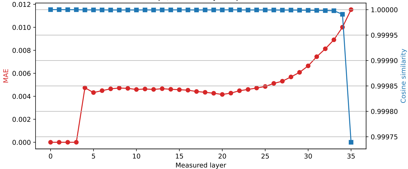
SmolLM3-3B | Quantized layer 3 | float32 \rightarrow int8
