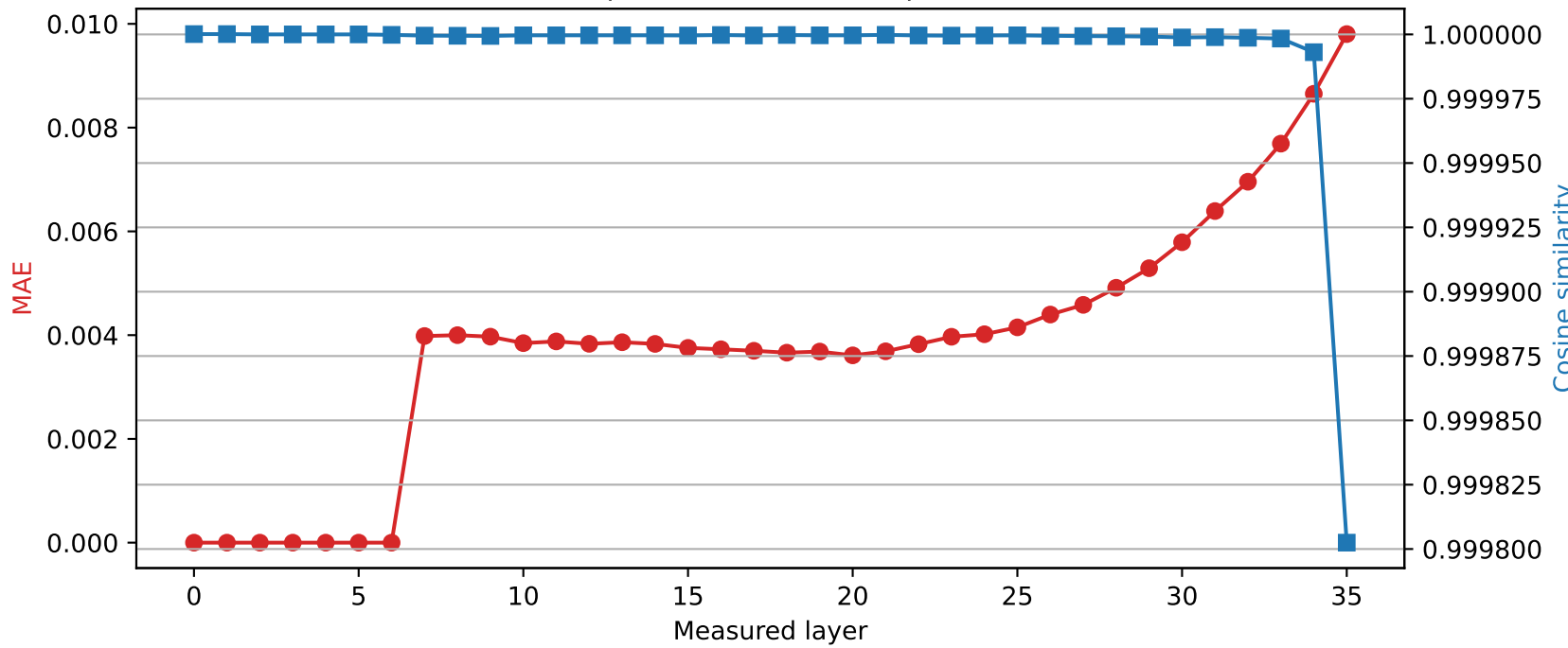
SmolLM3-3B | Quantized layer 6 | float32 \rightarrow int8
